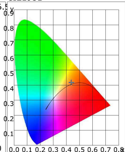
CIE1931
