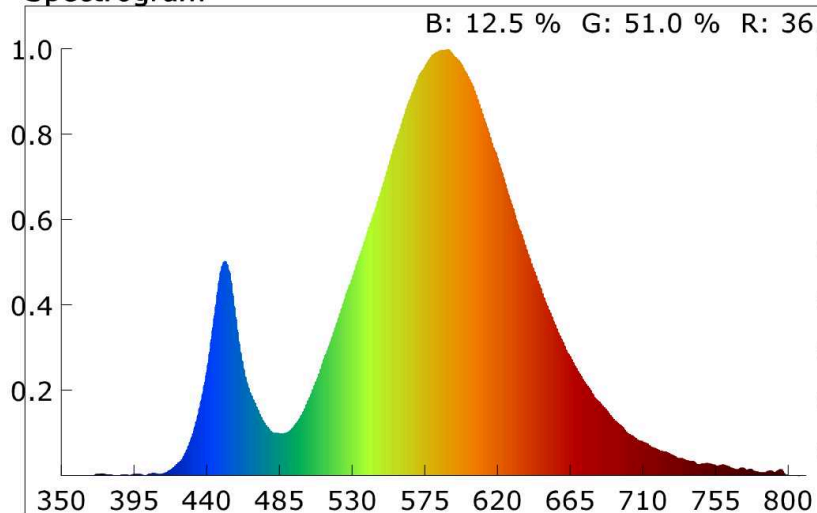
Spectrogram
